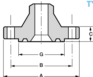
Welding-neck – WN
